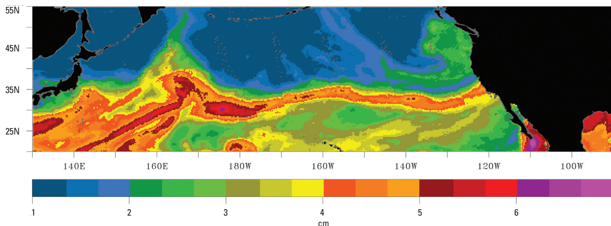
This satellite image from October 2009 shows an atmospheric river hitting the California coast. The color bar shows, in centimeters, the amount of water vapor in the air if all the water vapor were condensed into one layer of liquid. The light orange river in the middle registers nearly two inches. Image courtesy of Darren Jackson, NOAA/ESRL/PSD.
